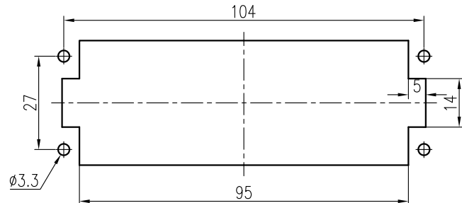
面板安装开孔图 Panel cut out
